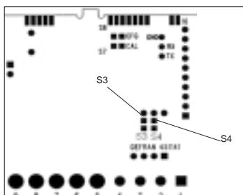
CPU board
